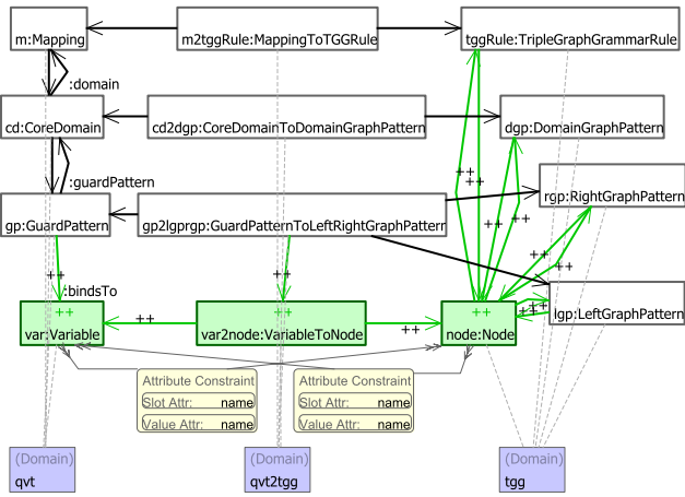
Fig. 21 Rule: GuardPatternVariableToNode
